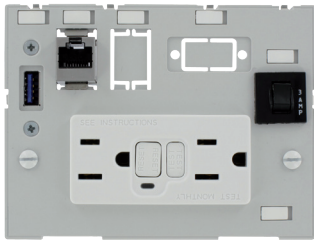
GFCI/RJ45/USB/3A Fuse 4000-68000-4100000
